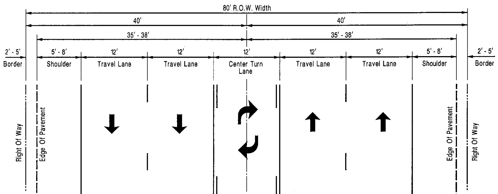
80' R.O.W. 5 LANE
